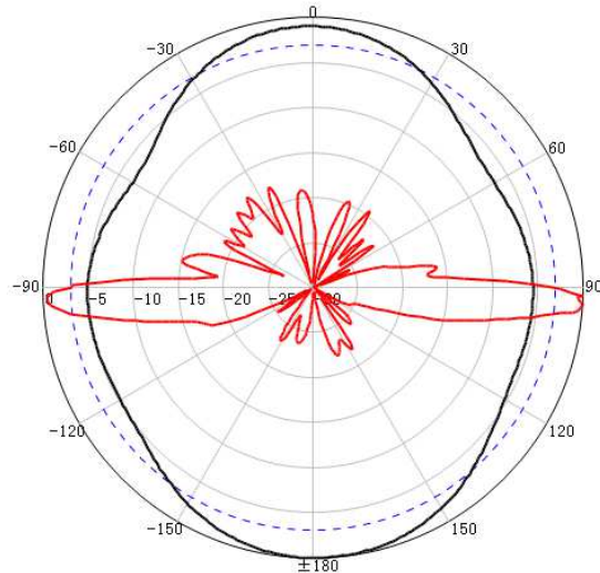
V-Pol @ 2450MHz
