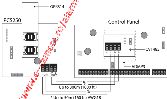
Figure 3: CVT485 Connection
